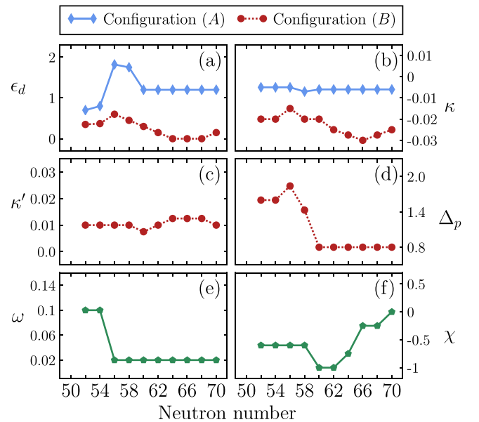
Figure 3. Parameters of the IBM-CM Hamiltonians, equations (10a), (10b), (11), are in MeV and the parameter \chi of equation (5), is dimensionless.
