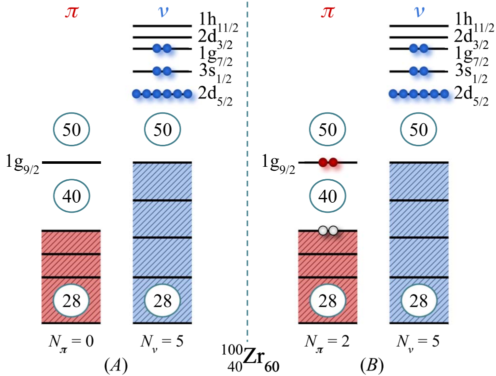
Figure 2. Schematic representation of the two coexisting shell-model configurations (A and B) for ^{100}\text{Zr}_{60} . The corresponding numbers of proton bosons ( N_\pi ) and neutron bosons ( N_\nu ), relevant to the IBM-CM, are listed for each configuration.
