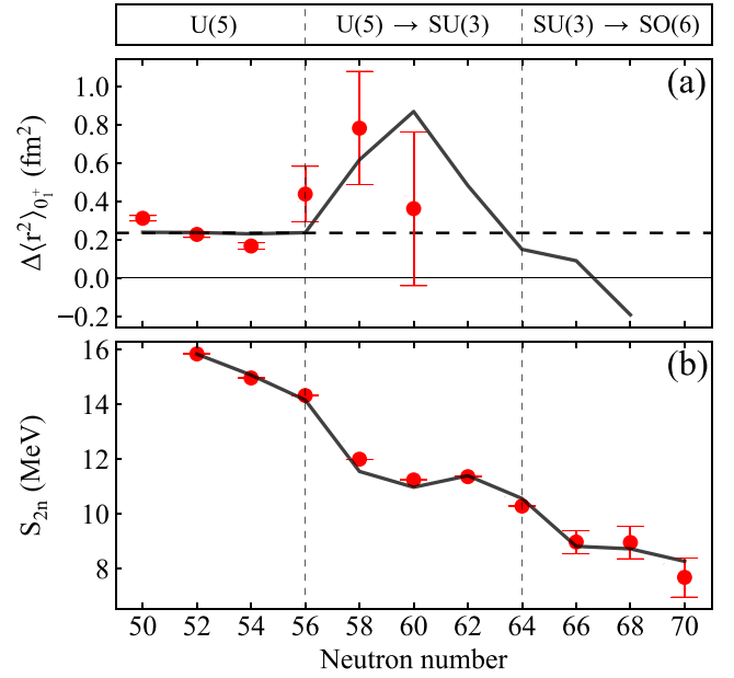
Figure 9. Evolution of observables along the Zr chain. Symbols (solid lines) denote experimental data (calculated results). (a) Isotope shift, \Delta \langle \hat{r}^2 \rangle_{0_1^+} in fm 2 . Data taken from [54]. The horizontal dashed line at 0.235 fm 2 represents the smooth behavior in \Delta \langle \hat{r}^2 \rangle_{0_1^+} due to the A^{1/3} increase of the nuclear radius. (b) Two-neutron separation energies, S_{2n} , in MeV. Data taken from AME2016 [55].
