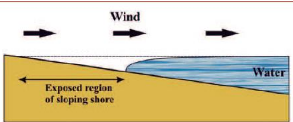
▲ Fig. 1: Diagram of wind setdown. The water is blown back, exposing a region of sloping shore (normal waterline drawn dotted).
