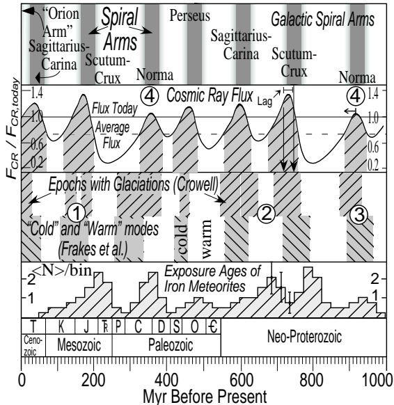
FIG. 1: The past Eon. Panel A describes past Galactic spiral arms crossings assuming \Delta\Omega = 10.9 \text{ (km s}^{-1}\text{)/kpc} . Panel B describes the CRF reaching the solar system using the CR diffusion model. Note that the CRF lags behind spiral arm crossings. This is portrayed by the hatched regions, which qualitatively show the predicted occurrences of IAEs if the CRF required to trigger them is the average flux. Arrows mark the middle of the spiral crossing and the expected mid-glaciation point. Panel C qualitatively describes the geologically recorded IAEs—its top half, as summarized by Crowell [25], who concluded that the current evidence is insufficient to support a claim of periodicity, while the bottom half, as summarized by Frakes et al. [26] who claim a periodicity exists. By fine tuning the observed pattern speed of the arms to best fit the IAEs, an intriguing correlation appears between the IAEs and their prediction. Note that the correlation need not be absolute since additional factors may affect the climate. Other factors that should be considered and noted in the graph are: (1) The mid-Mesozoic glaciations are significantly less extensive as others. (2) It is unclear to what extent was the period around 700 Myr BP warmer than the IAEs before or after. (3) The first IAE of the Neo-Proterozoic (if indeed distinct) is very uncertain. (4) Since Norma’s crossing is an extrapolation from smaller galactic radii, its location is uncertain. If the arm’s structure at smaller radii is indeed different [17], its preferred location will lag by about 20 Myr. Panel D is a 1-2-1 averaged histogram of the ^{41}\text{K}/^{40}\text{K} exposure ages of Fe Meteorites, which are predicted to cluster around the CRF minima. The cluster-IAE correlation further suggests an extra-terrestrial trigger for the glaciations.
