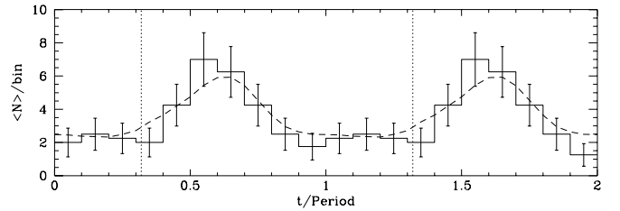
FIG. 2: A folded 1-2-1 averaged histogram (over the IAE periodicity) of the Fe Meteorites’ exposure ages. A statistically significant signal is obtained for a period of 143 \pm 10 \text{ Myr} . The dashed line is the CR diffusion model prediction. We find that the predicted phase of the cluster peaks, agrees with the actual exposure age clustering. The clustering peaks 100 Myr after the spiral crossing (dotted lines), implying that it is unlikely to be a real age clustering peak, which should be related directly to the spiral crossing (e.g., by Oort cloud comets being perturbed during arm crossing, that subsequently break asteroids more frequently, and that somehow affect the terrestrial climate).
